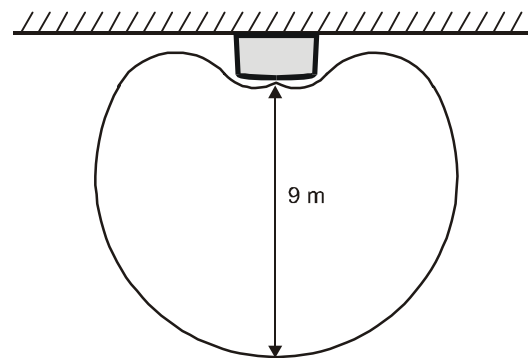
GBS-210 "VIVO" working range diagram
